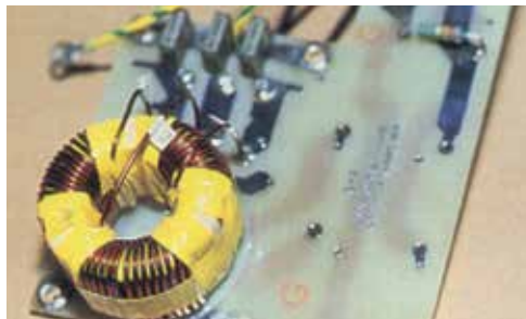
Coil outer wrap taping
